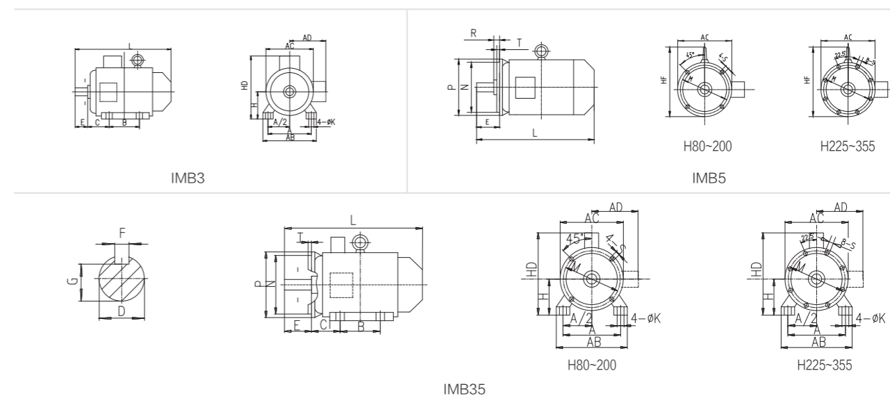
YE4 系列三相异步电动机安装及外形尺寸图 YE4 Series Motor Mounting and Overall Dimensions
